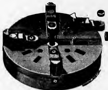
Front view of Chuck, showing manner of reversing the Jaws.
